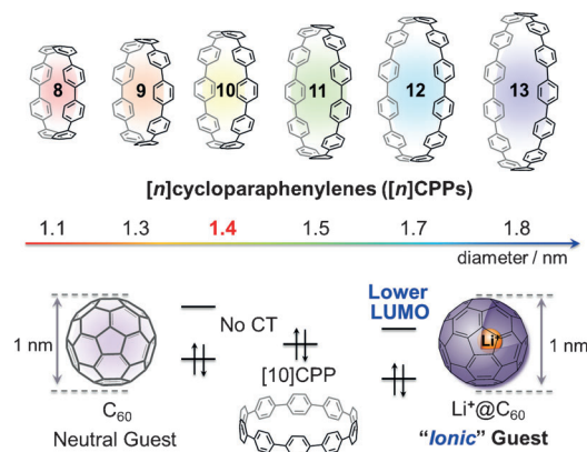
Figure 1. Top: Structures and diameters of cycloparaphenylenes ( n = 8 –13). Bottom: frontier molecular orbital energies of C_{60} and \text{Li}^+@C_{60} . The diameter of the [n]\text{CPPs} are taken from Ref. [3].
